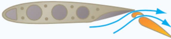
Slotted Fowler flap
